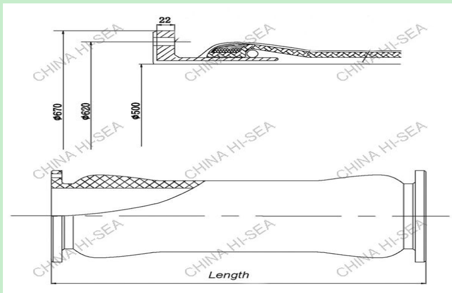
DN500 dredging discharge hose drawing
