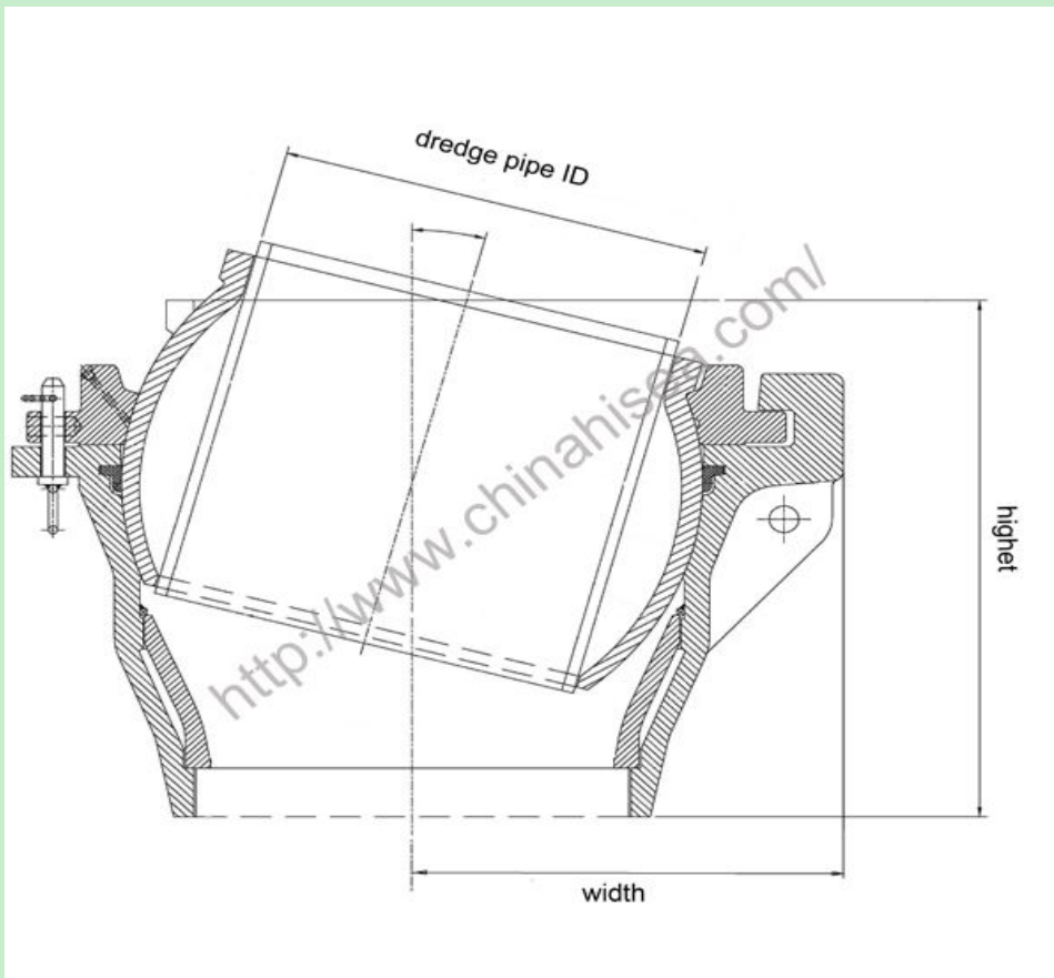
dredger ball joints drawing
