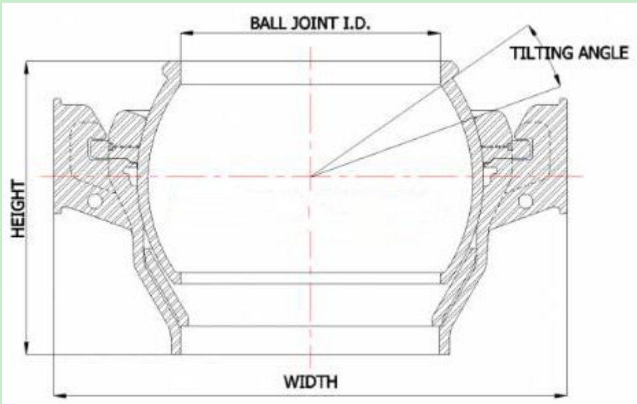
DN900 dredge ball joints drawing
