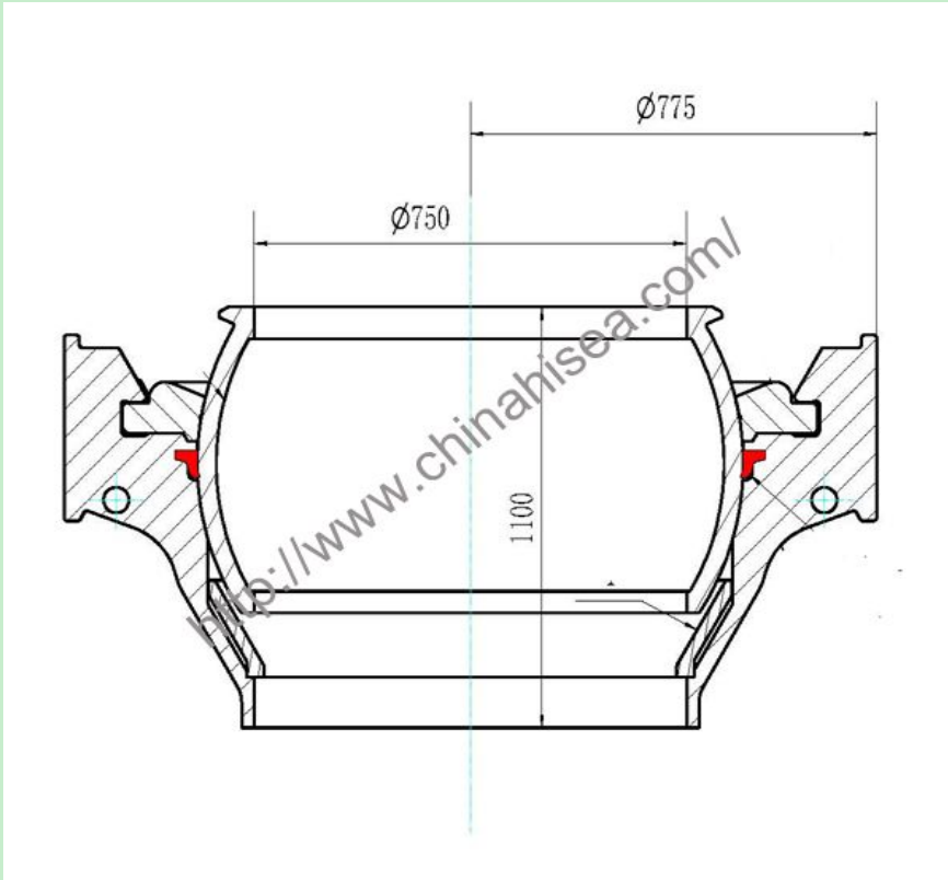
DN750 dredge ball joint drawing
