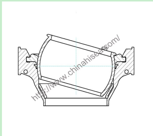
15° DN750 dredge ball joint
