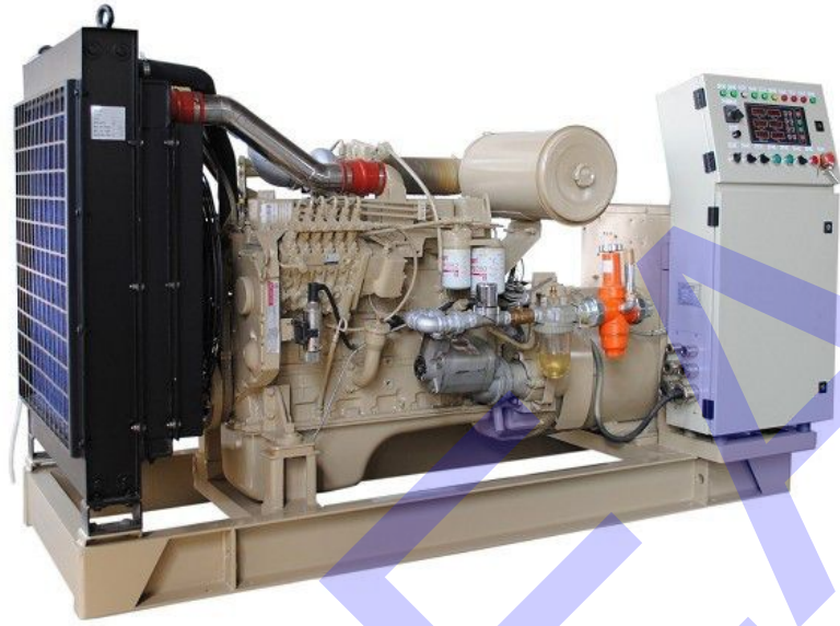
90kw cummins emergency marine diesel generator
