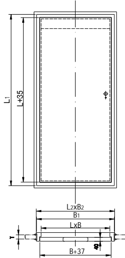
不带窗 WITHOUT WINDOW
