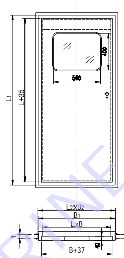
带双层窗 WITH DOUBLE WINDOW
