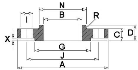
Slip-on flange
