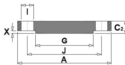
Blind flange
