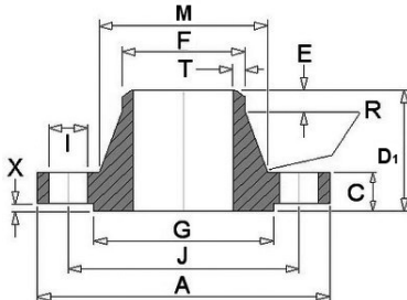
Weld neck flange
