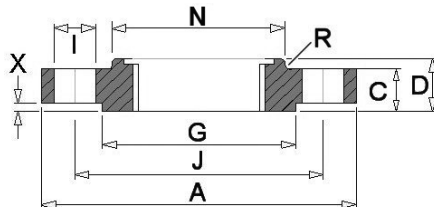
Socket welding flange
