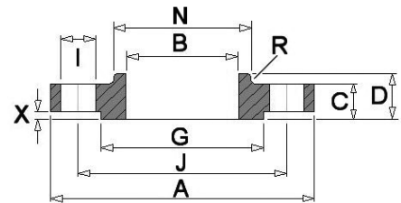
Slip-on flange
