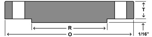
BLIND
