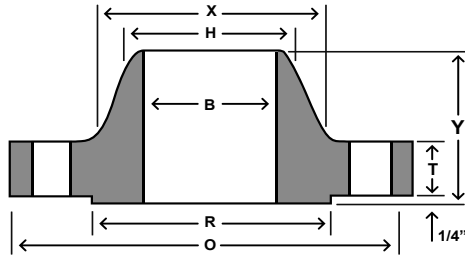
WELD NECK
