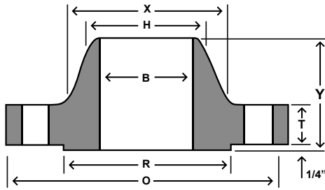
WELD NECK
