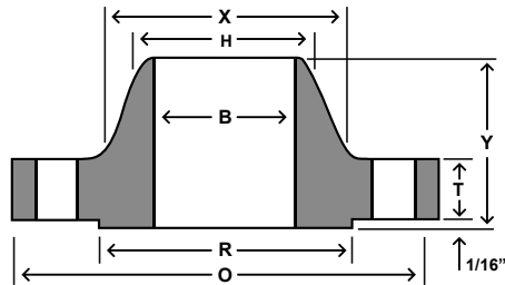
WELD NECK
