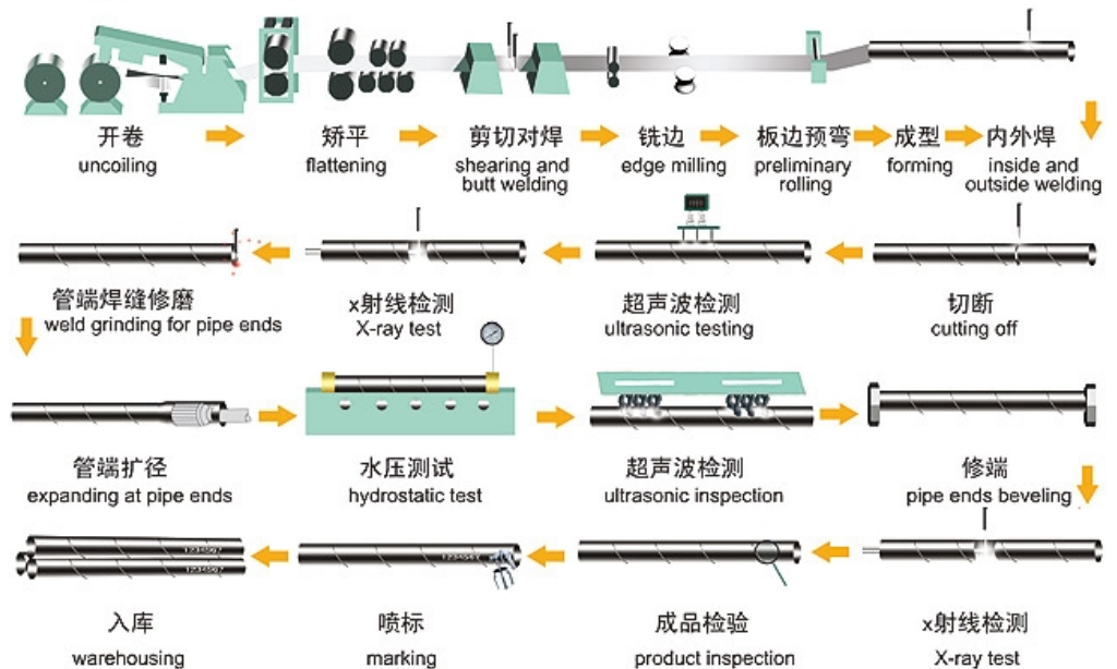
Manufacturing flow chart
