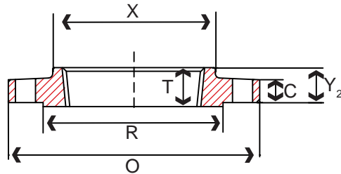
Stainless Steel Threaded Flange
