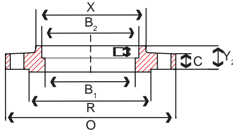
Stainless Steel Socket Weld Flange
