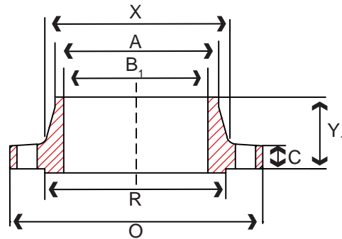
Stainless Steel Weld Neck Flange
